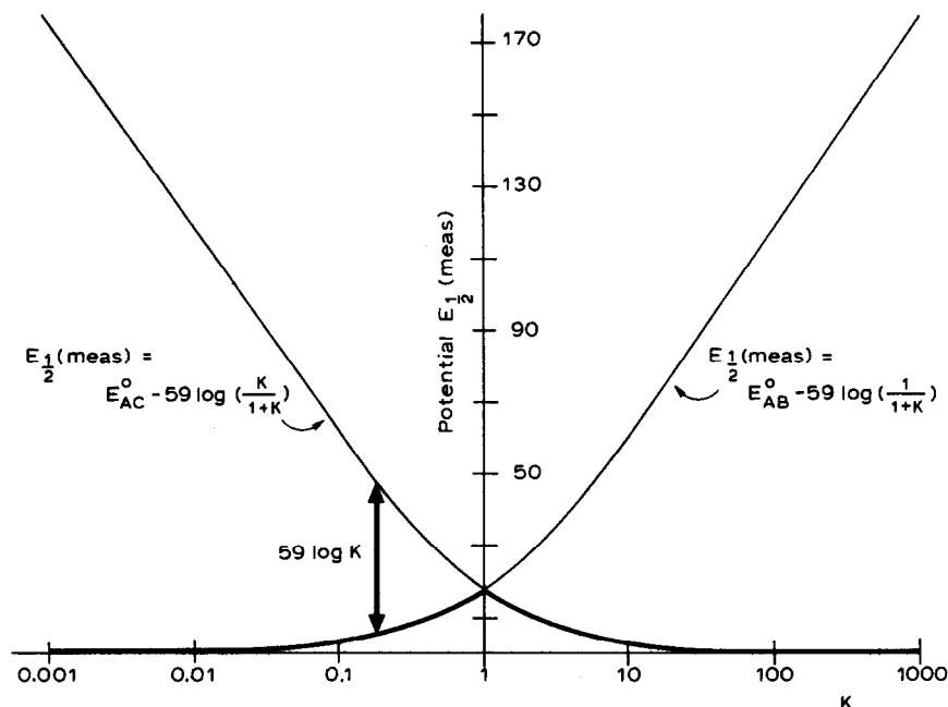
Fig. 24. Graphical plots of the relationships (in mV) E_{1/2}(\text{measured}) = E_{AC}^0 - 59 \log[K/(1+K)] and E_{1/2}(\text{measured}) = E_{AB}^0 - 59 \log[1/(1+K)] . It should be noted that each curve refers to a different reference potential, viz. E_{AC}^0 and E_{AB}^0 , respectively. Reproduced by courtesy: Inorg. Chem. , 14 (1975) 1894.
