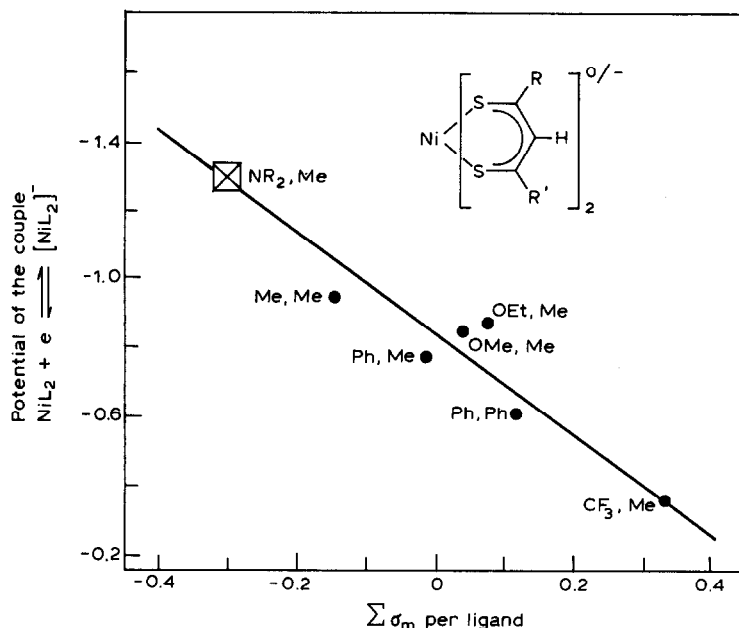
Fig. 20. Correlation between substituent effects (approximated by the Taft parameter \Sigma\sigma_m ) and the reduction potentials of Ni(R-Sac R'-Sac)_2 . Reproduced by courtesy: Inorg. Chem. , 15 (1976) 1118.
