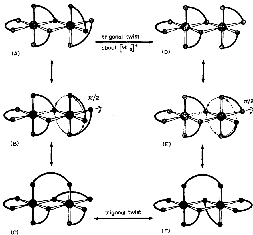
Fig. 9. A proposed mechanism for the interrelation of geometrical isomers for known binuclear cations of the type [\text{M}_2(\text{R}_2\text{dtc})_5]^+ . Structure (A), in which the two metal centres have opposite chiralities, may be converted into (D), where the metal chiralities are the same, by trigonal twist mechanism operating on the (\text{ML}_2)^+ segment of the cation. Rupture of a M-S bond (dotted), followed by a \pi/2 rotation along the indicated axis (structure (E)), and the reforming of a M-S(bridging) bond orthogonal to the ligand plane, affords isomeric structure (F). The presence of the metal-metal bond in the binuclear d^5 ruthenium cation may facilitate the spanning of the metal atoms by the unique [\text{R}_2\text{dtc}]^- ligand in structure (F). Reproduced by courtesy: Aust. J. Chem., 29 (1976) 269.
