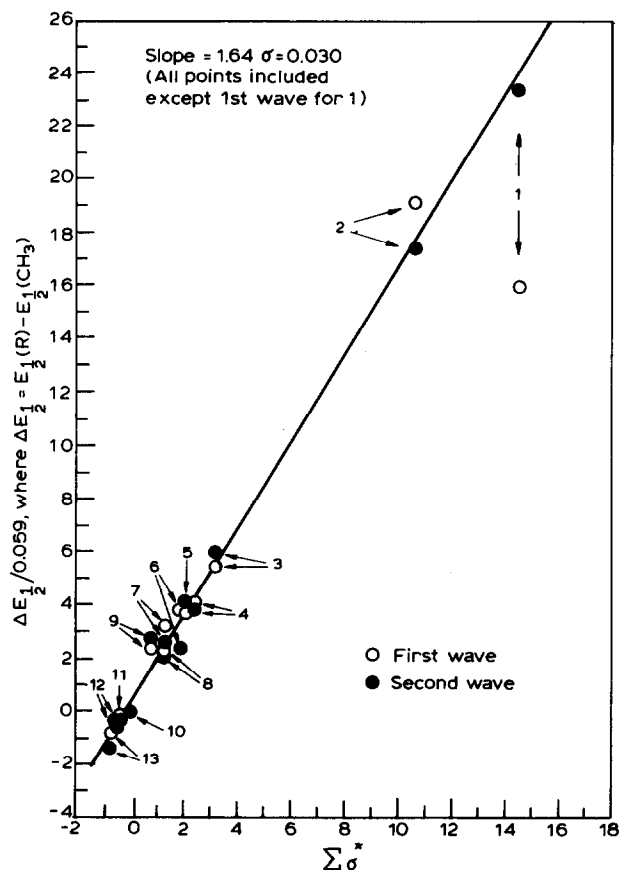
Fig. 21. Plot of \Delta E_{1/2} (0.059) vs. Taft's substituent constant weighted for number of R groups present for \text{Ni}(\text{S}_4\text{C}_4\text{R}_4) complexes. R = 1, CN; 2, \text{CF}_3 ; 3, p\text{-C}_6\text{H}_4\text{Cl} ; 4, \text{C}_6\text{H}_5 ; 5, \text{NiS}_4\text{C}_4\text{Ph}_2\text{H}_2 ; 6, H; 7, p\text{-C}_6\text{H}_4\text{CH}_3 ; 8, \text{NiS}_4\text{C}_4(\text{CH}_3)_2\text{Ph}_2 ; 9, p\text{-C}_6\text{H}_4\text{OCH}_3 ; 10, \text{CH}_3 ; 11, \text{C}_2\text{H}_5 ; 12, n\text{-C}_3\text{H}_7 ; 13, i\text{-C}_3\text{H}_7 . Reproduced by courtesy: Transition Met. Chem. , 4 (1968) 299.
