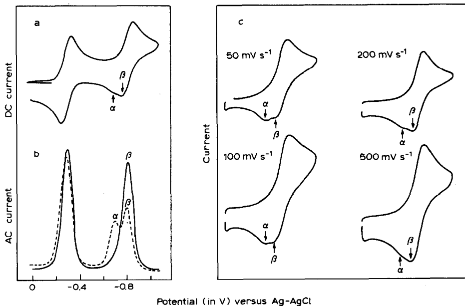
Fig. 8. (a) Cyclic voltammogram of \beta - [\text{Ru}_2(\text{Me}_2\text{dtc})_3][\text{BF}_4] in acetone (0.1 M \text{Et}_4\text{NClO}_4 ) (scan rate 200 \text{mV s}^{-1} ). (b) Cyclic a.c. voltammogram (solution as in (a)): (—), negative scan; (---), positive scan obtained by holding a negative potential for ca. 10 s. Scan rate 100 \text{mV s}^{-1} . In both (a) and (b) the second reduction process displays the \beta^- \rightarrow \alpha^- isomerization of the anion. (c) Effect of scan rate on the \beta^- \rightarrow \alpha^- isomerization of [\text{Ru}_2(\text{Me}_2\text{dtc})_5]^- Complex added to acetone (0.1 M \text{Et}_4\text{NClO}_4 ) solution as \beta - [\text{Ru}_2(\text{Me}_2\text{dtc})_5]\text{Cl} . Redox processes centered at ca. -0.75 V vs. \text{Ag}/\text{AgCl} . Reproduced by courtesy: J. Chem. Soc., Dalton Trans. (1976) 2032.
