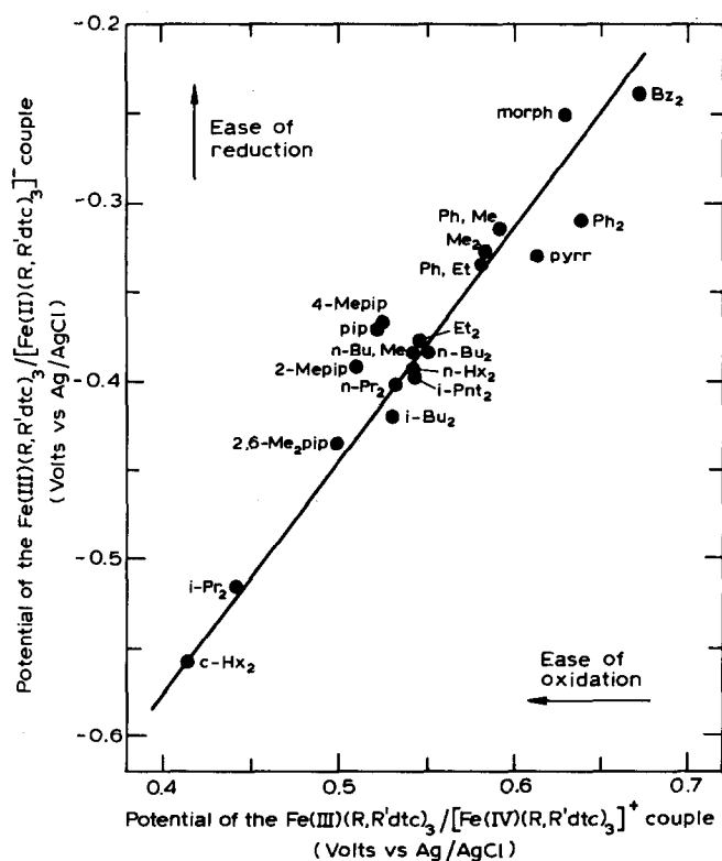
Fig. 6. Relation between the oxidation and reduction potentials of \text{Fe}(\text{RR'dtc})_3 complexes. Reproduced by courtesy: Inorg. Chem. , 14 (1975) 1894.
