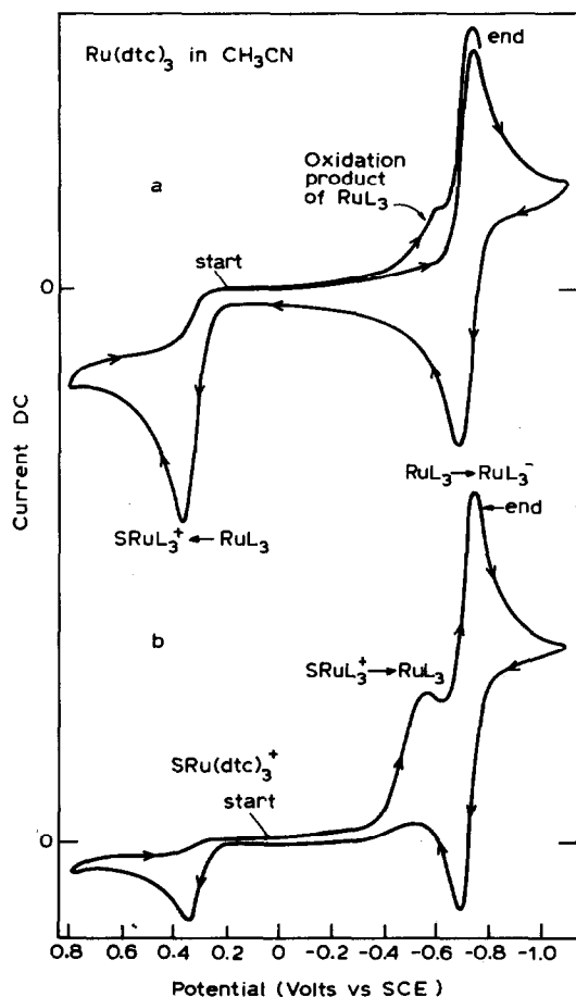
Fig. 7. (a) Cyclic voltammogram of \text{Ru}(\text{Et}_2\text{dte})_3 in \text{CH}_3\text{CN} (ca. 0.1 M \text{Et}_4\text{NClO}_4 ) (scan rate 200 \text{ mV s}^{-1} ). (b) Cyclic voltammogram of the above solution in (a) after controlled-potential electrolysis at 0.50 V vs. SCE. Approximately 85% of the \text{Ru}(\text{Et}_2\text{dte})_3 has been oxidized. Reproduced by courtesy: Inorg. Chem. , 17 (1978) 340.
