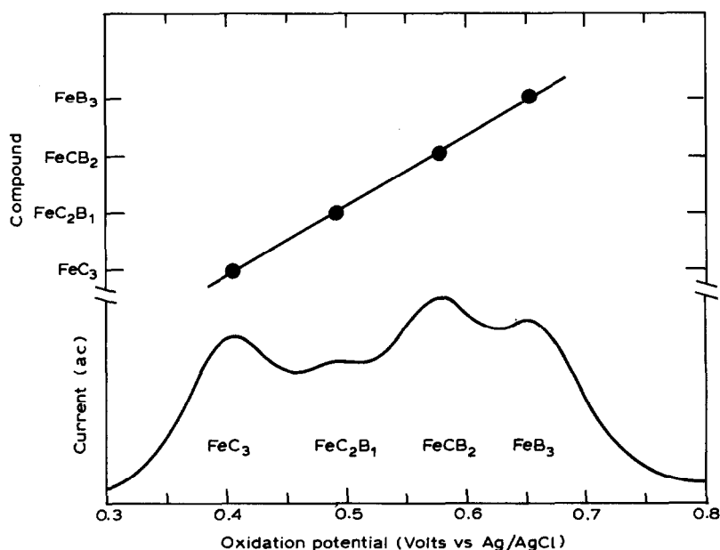
Fig. 5. Bottom curve: a.c. voltammogram (oxidation) of a solution containing a mixture of mixed-ligand species \text{FeC}_3 , \text{FeC}_2\text{B} , \text{FeCB}_2 , and \text{FeB}_3 where C = dicyclohexyldithiocarbamate and B = dibenzylidithiocarbamate. Top curve: relationship between complex composition and a.c. peak potential. Reproduced by courtesy: Inorg. Chem., 14 (1975) 1894.
